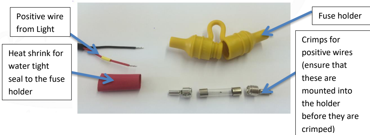
Fig 4 showing how the Gel connector is wired up.
